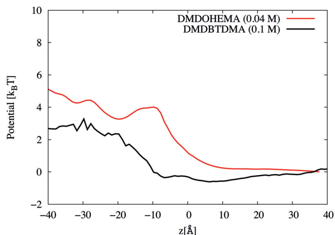
Figure 3. Interfacial potential in k_B T units across the oil–water interface for neodymium considering either DMDOHEMA or EXT1 (at 0.04 \text{ mol L}^{-1} ) or DMDBTDMA or EXT2 (at 0.1 \text{ mol L}^{-1} ). These concentrations correspond approximatively to the CAC for both systems.
